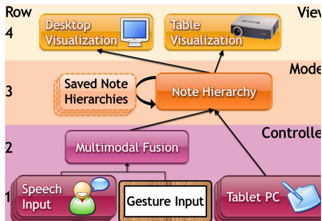
Figure 8. The Designers’ Environment architecture
